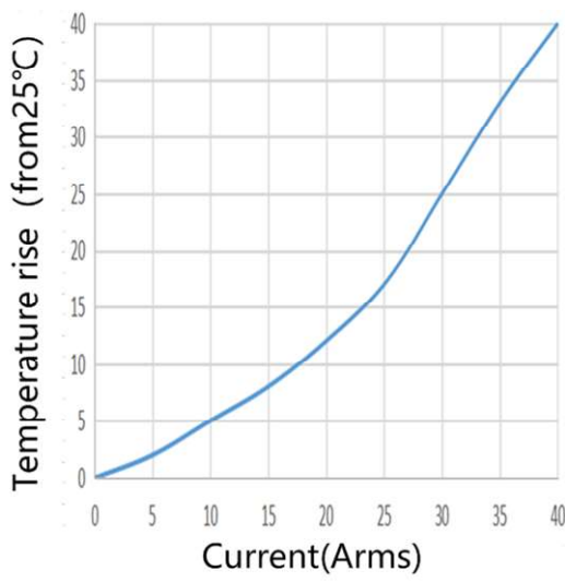
Temperature Rise vs Current
