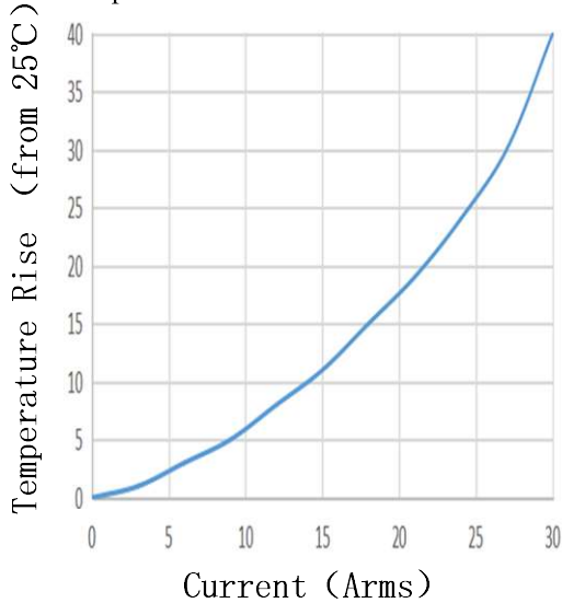
Temperature Rise vs Current
